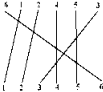
Figure 2. Permutations of 123456.
