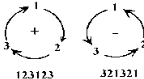
Figure 1. Permutations of 123.
